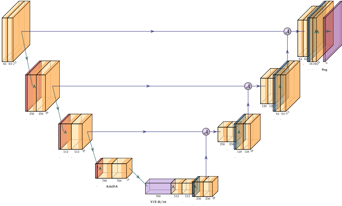
Fig. 1. ApproxDA-TransUNet architecture. ApproxDABlocks (Low-Rank Windowed PAM + Grouped CAM + gate routing) replace dual-attention modules at all skip connections and the bottleneck. gate_mode controls the routing during ablation.
