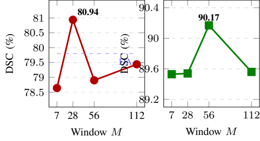
Fig. 4. DSC vs. window size M (gate=pam, r=32 ). Left (Synapse, high CS): non-monotonic curve, peak at M=28 (+1.14% vs. DA-TransUNet, dashed blue), range 2.30%. Right (Kvasir-SEG, low CS): near-flat plateau, range 0.64%. The 3.6\times sensitivity ratio operationalizes CS empirically.
