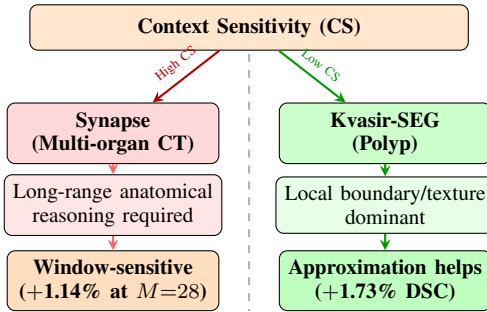
Fig. 9. Context Sensitivity (CS) governs approximation window importance. All three tasks benefit from ApproxDA (+1.14% Synapse at M=28 ; +1.73% Kvasir at M=56 ; +1.15% ISIC at M=7 ), but performance sensitivity to window choice is 3.6\times higher on the high-CS benchmark (Synapse CS=2.30 pp vs. Kvasir CS=0.64 pp). ISIC CS (window ablation pending) follows the low-CS pattern.
