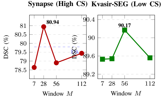
Fig. 4. DSC vs. window size M (gate=pam, r=32 ). Left (Synapse, high CS): non-monotonic curve, peak at M=28 (+1.14% vs. DA-TransUNet, dashed blue), range 2.30%. Right (Kvasir-SEG, low CS): near-flat plateau, range 0.64%. The 3.6\times sensitivity ratio operationalizes CS empirically.
