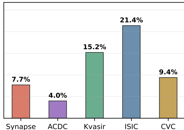
SC1: Foreground Ratio (expect \rho \approx 0 )
