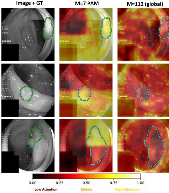
Fig. 5. PAM contribution maps ( \| \text{output} - \text{input} \|_2 , per-panel normalised; colorbar below) on three Kvasir-SEG polyp images. Each row: input with GT contour (left), windowed PAM ( M=7 ; center), global PAM ( M=112 ; right). Brighter color indicates larger PAM contribution at that location; panels are independently normalised so magnitudes are not comparable across panels.
