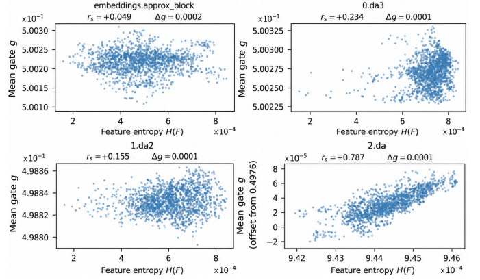
Fig. 6. Gate value g vs. feature entropy H(F) at all four skip locations ( M=7 , \text{gate=learn} ): bottleneck, 28^2 , 56^2 , 112^2 . All cluster at g \approx 0.5 ( \Delta g \leq 0.0002 ), confirming gate collapse.
