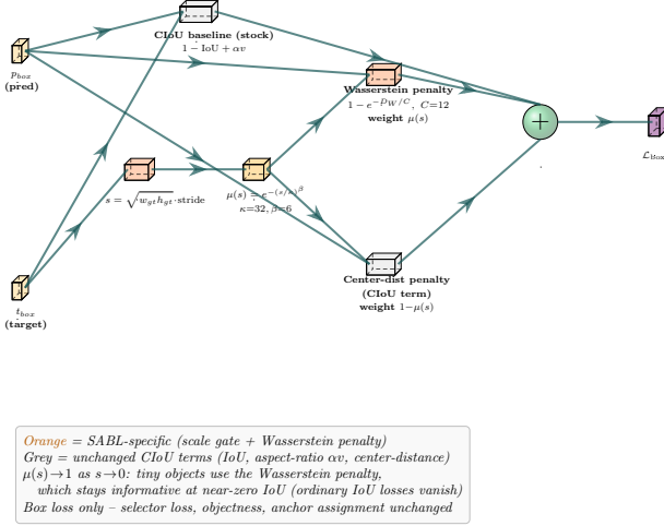
Fig. 3. Illustration of the Scale-Aware Balancing Loss (SABL). The scale gating function \mu(s) adaptively balances the Normalized Gaussian Wasserstein distance for micro-scale targets and CIoU for larger objects.
