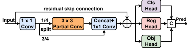
Fig. 3. Inverted Residual Decoupled Head (ISPP) with Partial Convolution (© denotes channel concatenation).
