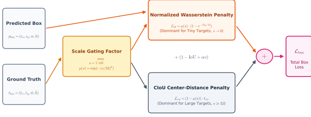
Fig. 3. Illustration of the Scale-Aware Balancing Loss (SABL). The scale gating function \mu(s) adaptively balances the Normalized Gaussian Wasserstein distance for micro-scale targets and CIoU for larger objects.
