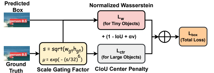
Fig. 3. Scale-Aware Balancing Loss (SABL) workflow.
