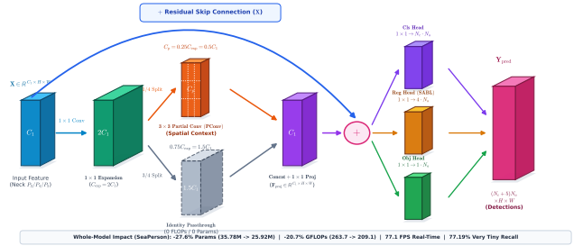
Fig. 2. Architecture of the Inverted Residual Decoupled Head (ISPPHead) with Partial Convolution.
