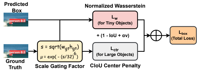
Fig. 3. Scale-Aware Balancing Loss (SABL) workflow.
