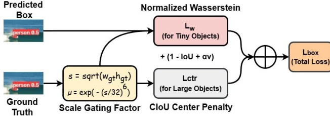
Fig. 3. Scale-Aware Balancing Loss (SABL) workflow (§3.3).
