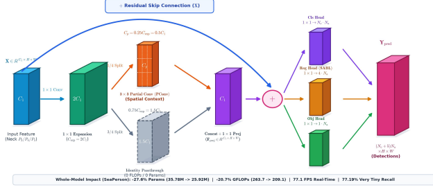
Fig. 2. Architecture of the Inverted Residual Decoupled Head (ISPPHead) with Partial Convolution (§3.3).
