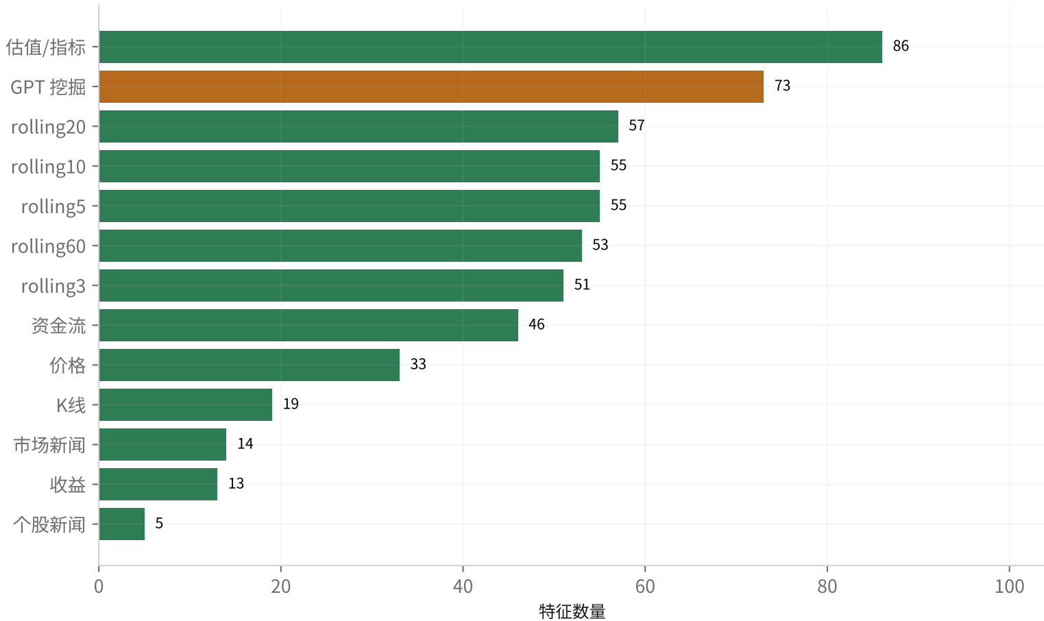
reviewed 入选特征分布 (n=560)
