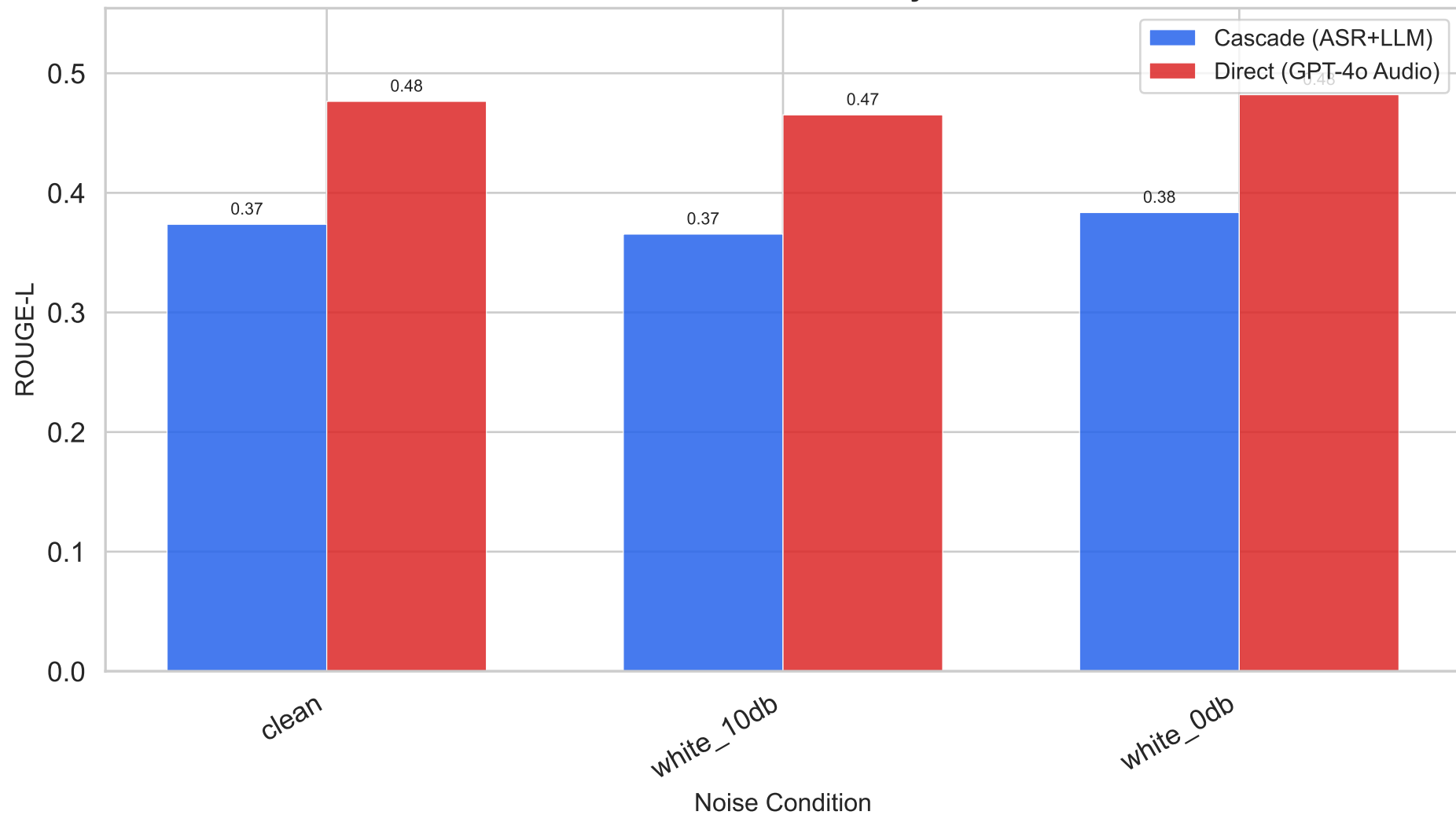
Robustness: Summarization Quality vs White Noise
