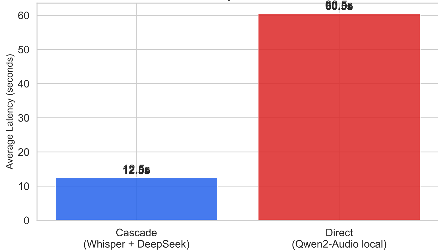
Inference Latency: Cascade vs Direct
