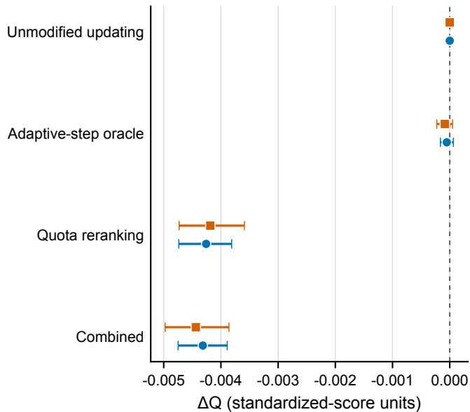
(b) Change in accepted-item score
