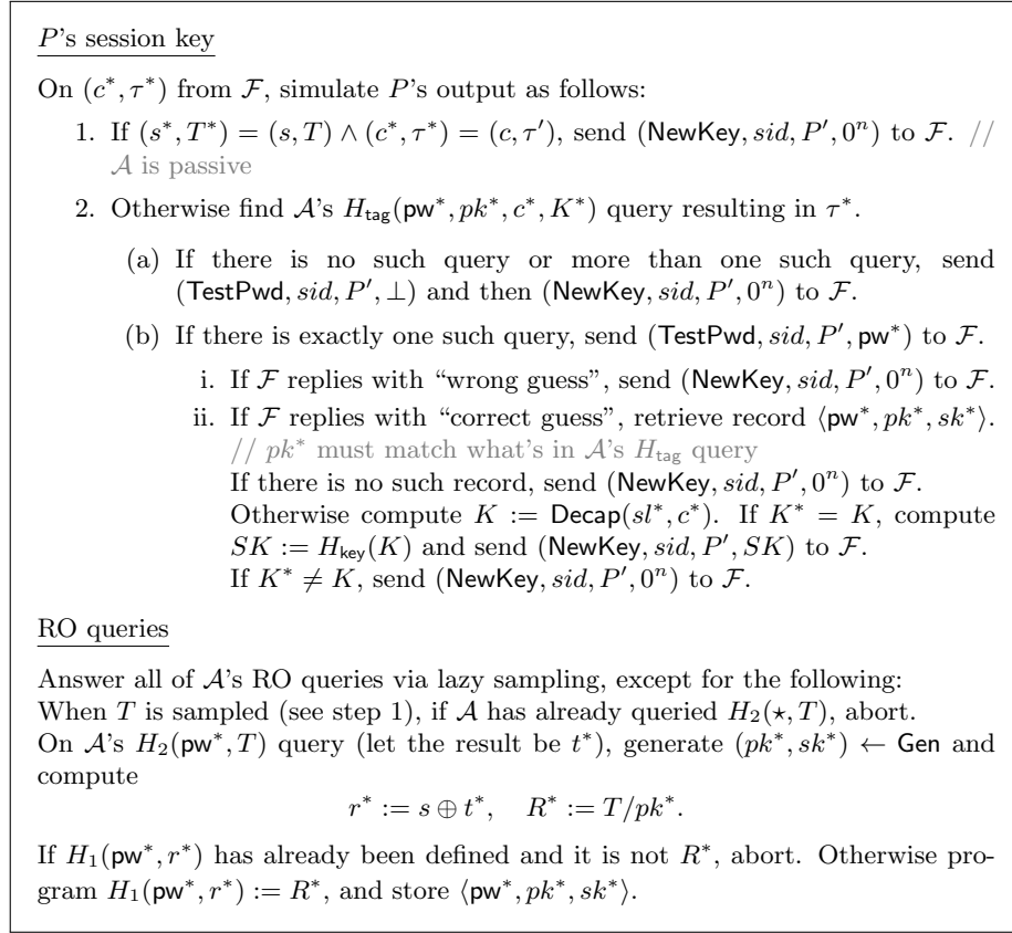
Figure 2: UC simulator \mathcal{S} for OEKE (part 2)
