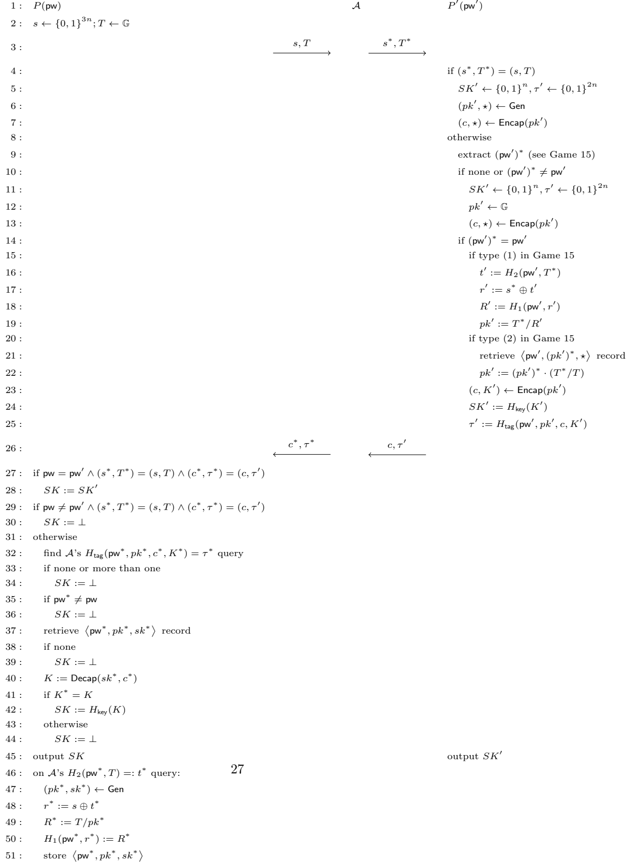
Figure 4: Game 17 (with various aborting conditions omitted)
