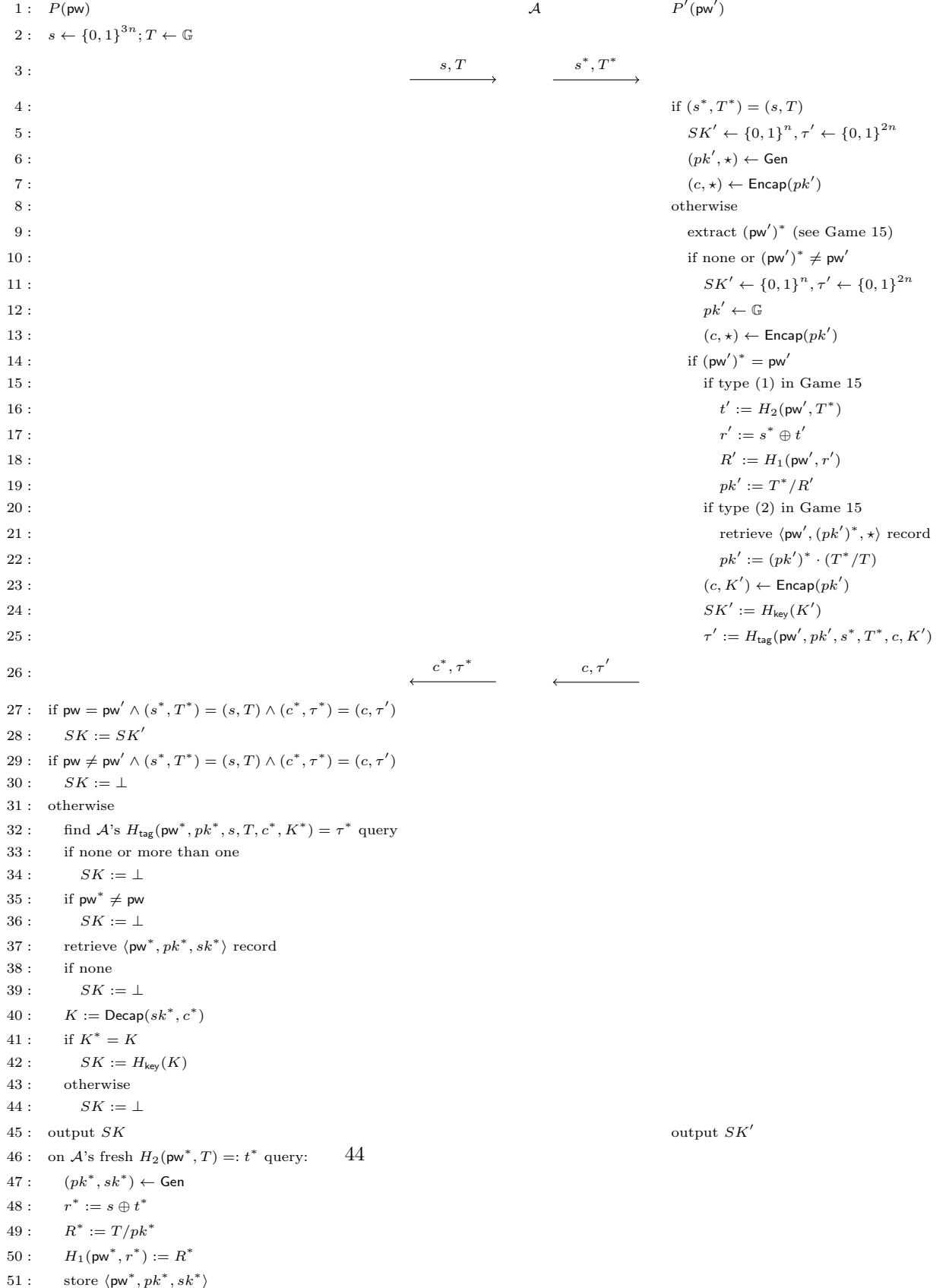
Figure 7: Game 17 (with various aborting conditions omitted)
