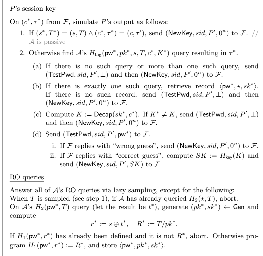
Figure 3: UC simulator \mathcal{S} for OEKE (part 2)
