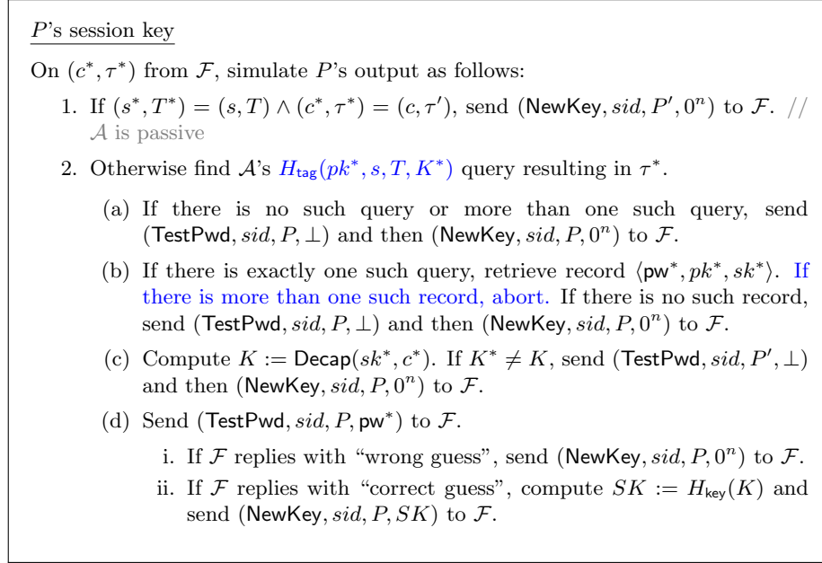
Figure 7: UC simulator \mathcal{S} for the “hash pk and (s, T) ” variant of OEKE. Only the paragraph that needs significant change (shown in blue) is included
