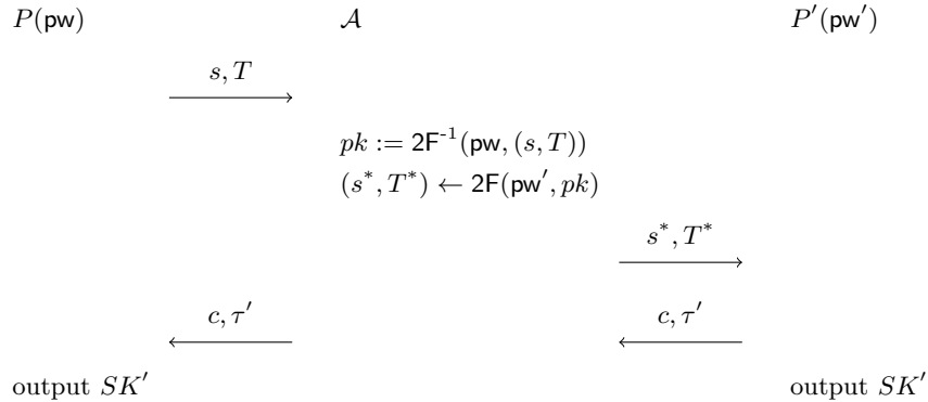
Figure 14: New “attack” on the “hash pk ” version
