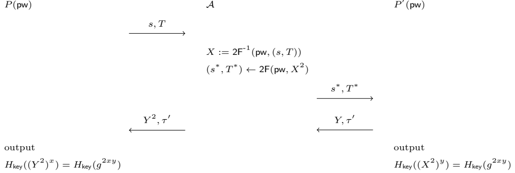
Figure 12: New “attack” on the “hash \text{pw} ” version, using OEKE based on Diffie–Hellman KEM
