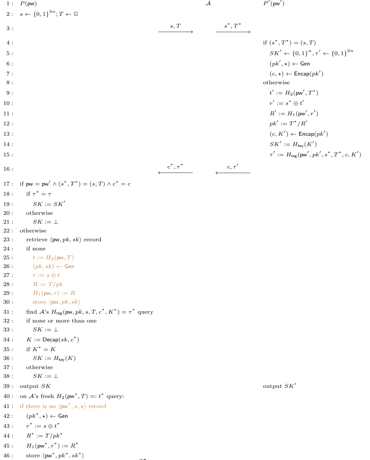
Figure 6: Game 10 (with various aborting conditions omitted)
