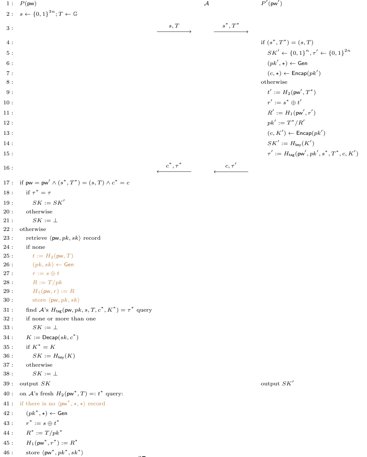
Figure 7: Game 10 (with various aborting conditions omitted)
