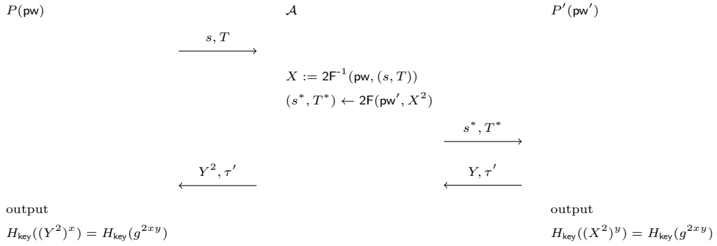
Figure 17: New “attack” on the “hash \text{pw} ” version, using OEKE based on Diffie–Hellman KEM
