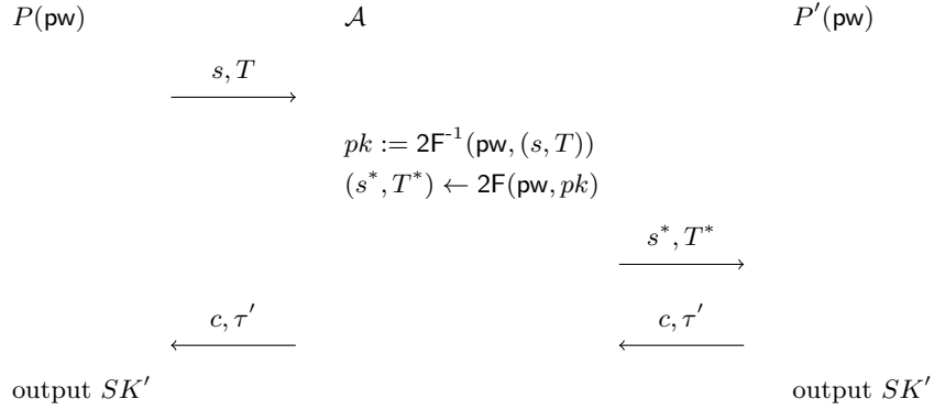
Figure 11: New “attack” on the “hash \text{pw} and pk ” version
