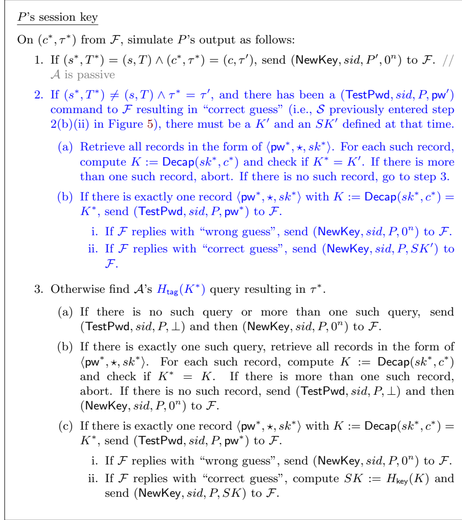
Figure 18: UC simulator \mathcal{S} for the “hash pk ” variant of OEKE. Only the paragraph that needs essential change from Figure 10 (shown in blue) is included
