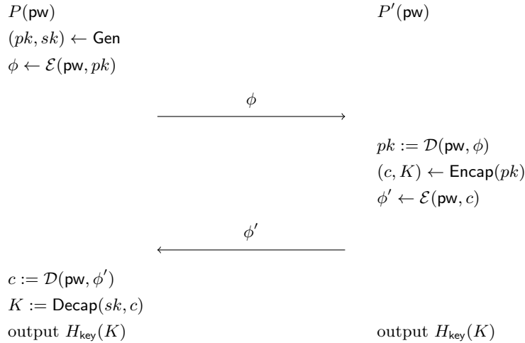
Figure 1: The EKE protocol with KEM scheme (\text{Gen}, \text{Encap}, \text{Decap}) and symmetric encryption (\mathcal{E}, \mathcal{D})
