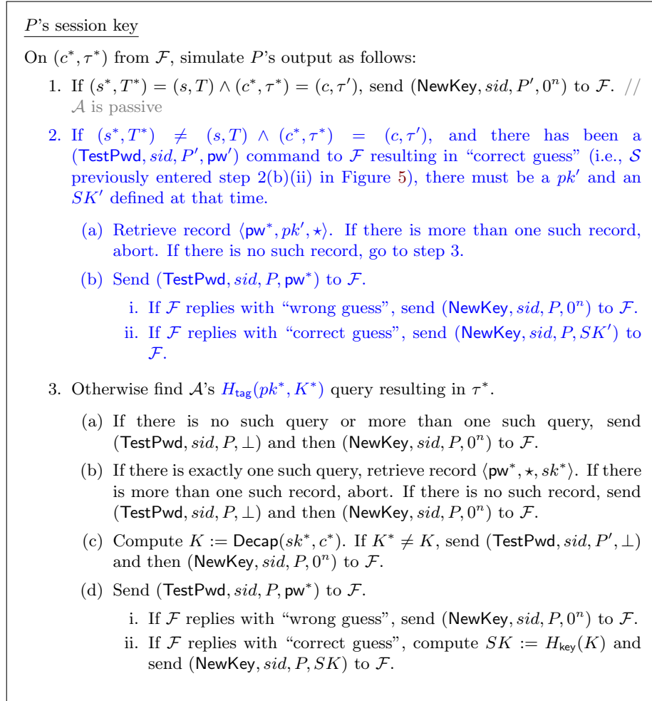
Figure 16: UC simulator \mathcal{S} for the “hash pk ” variant of OEKE. Only the paragraph that needs essential change from Figure 9 (shown in blue) is included
