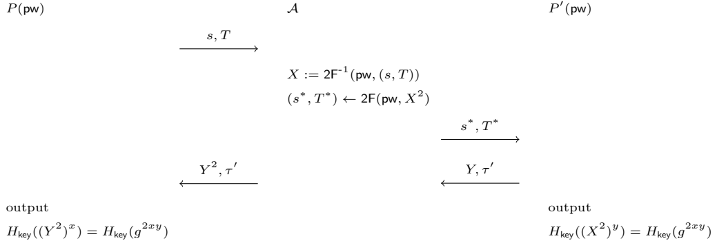
Figure 13: New “attack” on the “hash pw” version, using OEKE based on Diffie–Hellman KEM
