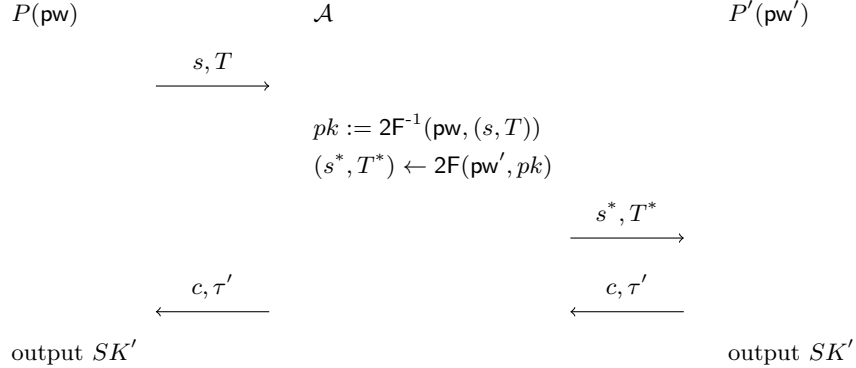
Figure 15: New “attack” on the “hash pk ” version
