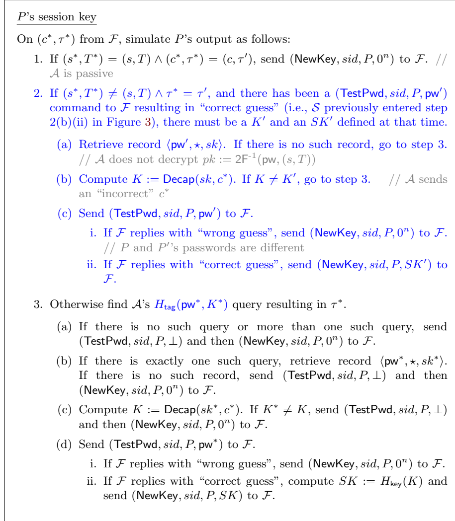
Figure 12: UC simulator \mathcal{S} for the “hash pk ” variant of OEKE. Only the paragraph that needs essential change (shown in blue) is included
