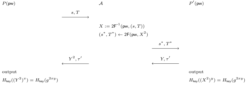
Figure 11: New “attack” on the “hash \text{pw} ” version, using OEKE based on Diffie–Hellman KEM
