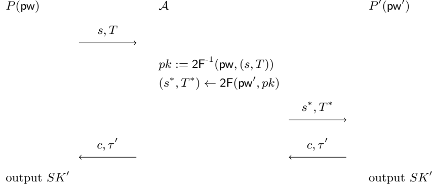
Figure 13: New “attack” on the “hash pk ” version
