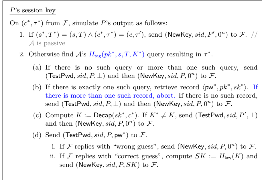
Figure 7: UC simulator \mathcal{S} for the “hash pk and (s, T) ” variant of OEKE. Only the paragraph that needs essential change (shown in blue) is included
