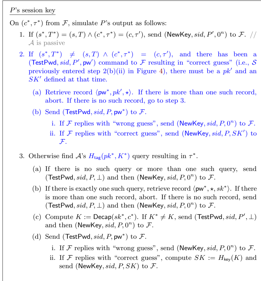
Figure 15: UC simulator \mathcal{S} for the “hash pk ” variant of OEKE. Only the paragraph that needs essential change from Figure 8 (shown in blue) is included
