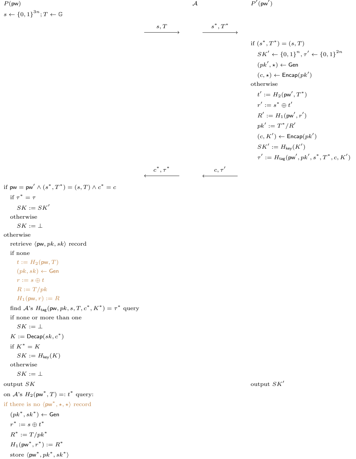
Figure 5: Game 10 (with various aborting conditions omitted)
