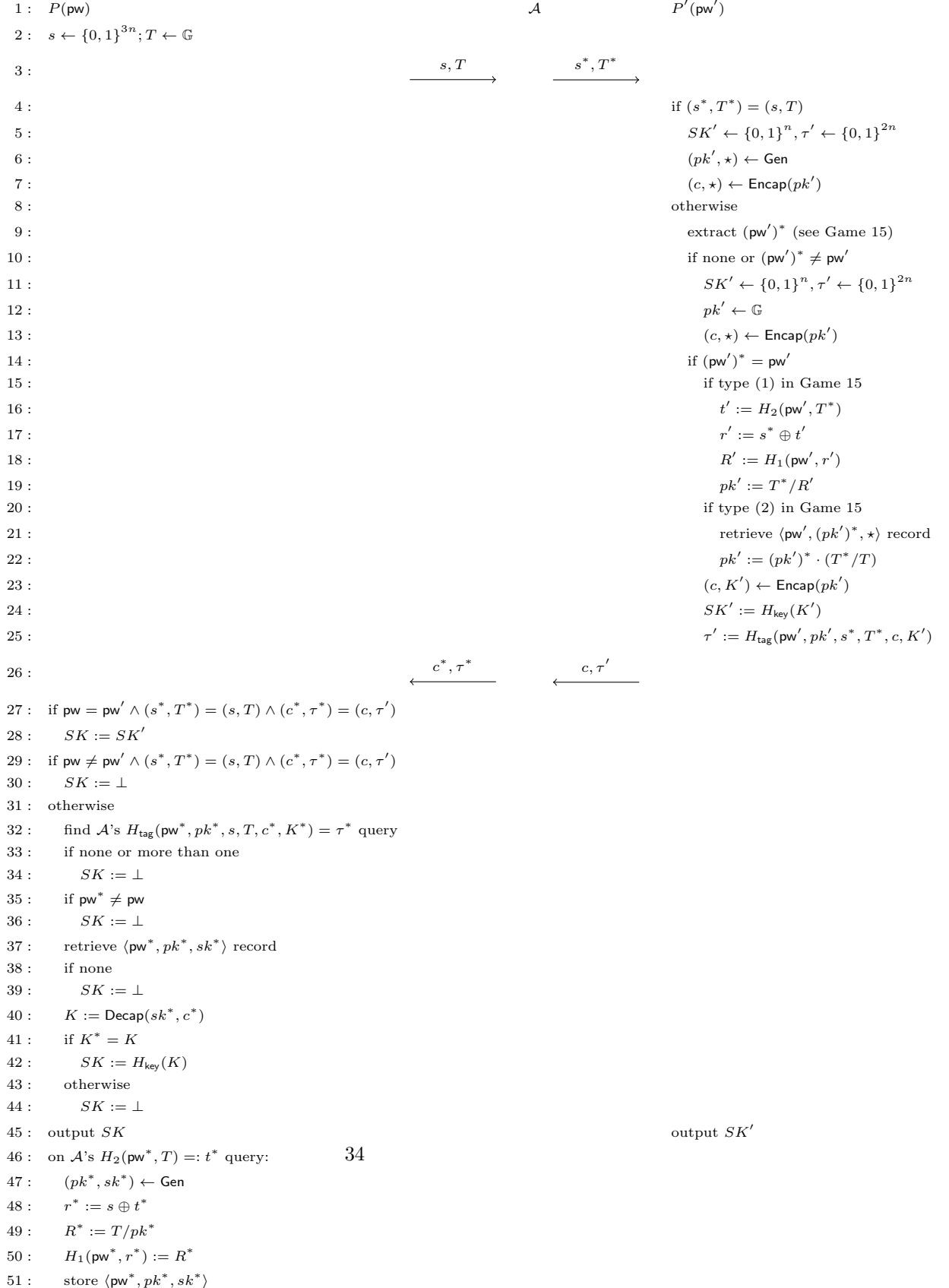
Figure 6: Game 17 (with various aborting conditions omitted)
