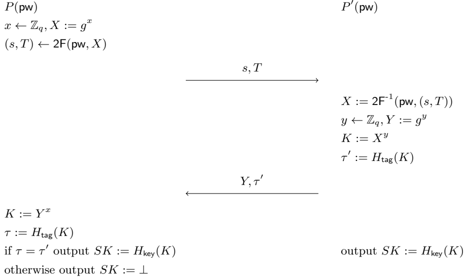
Figure 3: The OEKE-2F protocol with Diffie–Hellman KEM
