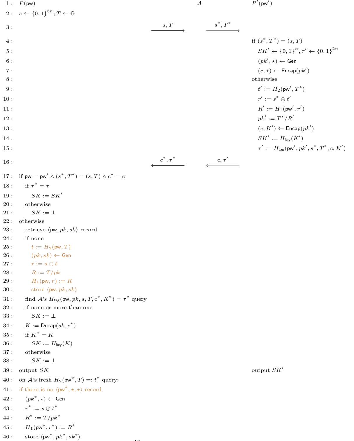
Figure 8: Game 10 (with various aborting conditions omitted)
