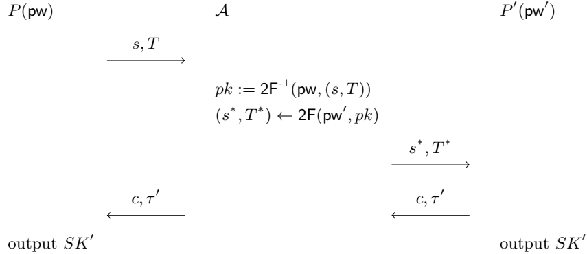
Figure 16: New “attack” on the “hash pk ” version
