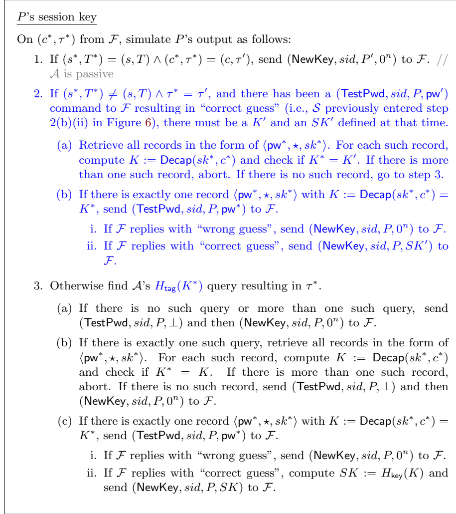
Figure 19: UC simulator \mathcal{S} for the “hash pk ” variant of OEKE. Only the paragraph that needs essential change from Figure 11 (shown in blue) is included
