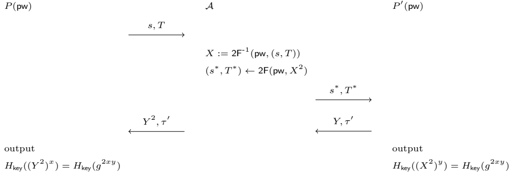
Figure 14: New “attack” on the “hash pw” version, using OEKE based on Diffie–Hellman KEM
