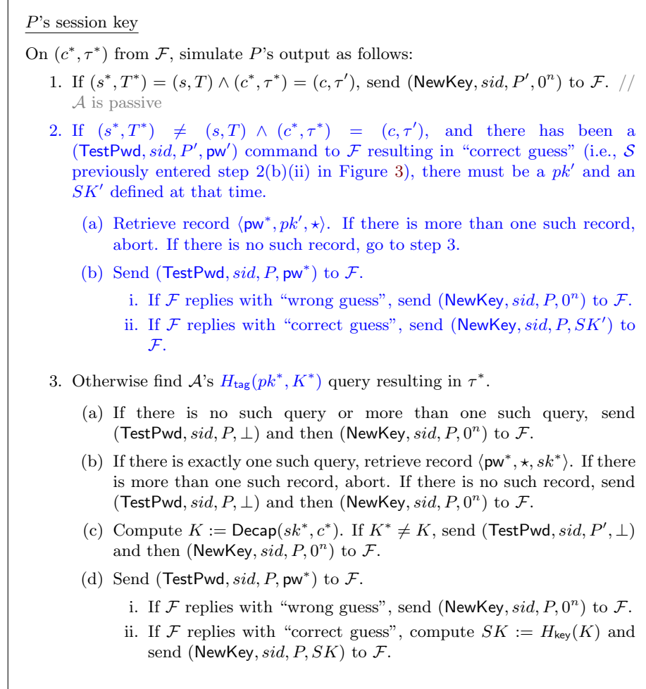
Figure 12: UC simulator \mathcal{S} for the “hash pk ” variant of OEKE. Only the paragraph that needs essential change from Figure 7 (shown in blue) is included
