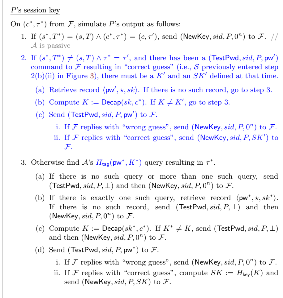
Figure 10: UC simulator \mathcal{S} for the “hash pk ” variant of OEKE. Only the paragraph that needs essential change (shown in blue) is included
