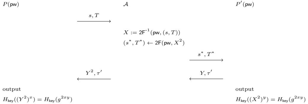
Figure 11: New “attack” on the “hash \text{pw} ” version, using OEKE based on Diffie–Hellman KEM
