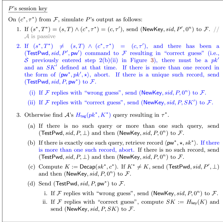
Figure 12: UC simulator \mathcal{S} for the “hash pk ” variant of OEKE. Only the paragraph that needs significant change (shown in blue) is included
