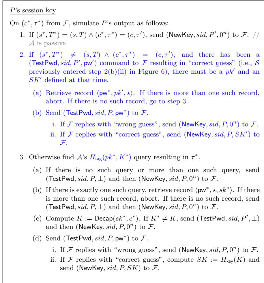
Figure 17: UC simulator \mathcal{S} for the “hash pk ” variant of OEKE. Only the paragraph that needs essential change from Figure 10 (shown in blue) is included
