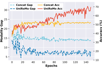
(a) Clean: Joint
