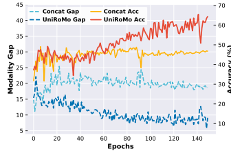
(b) Hybrid: Joint
