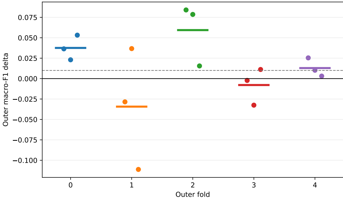
Mature operator counterfactual: MBConv-5x5 vs MBConv-3x3
