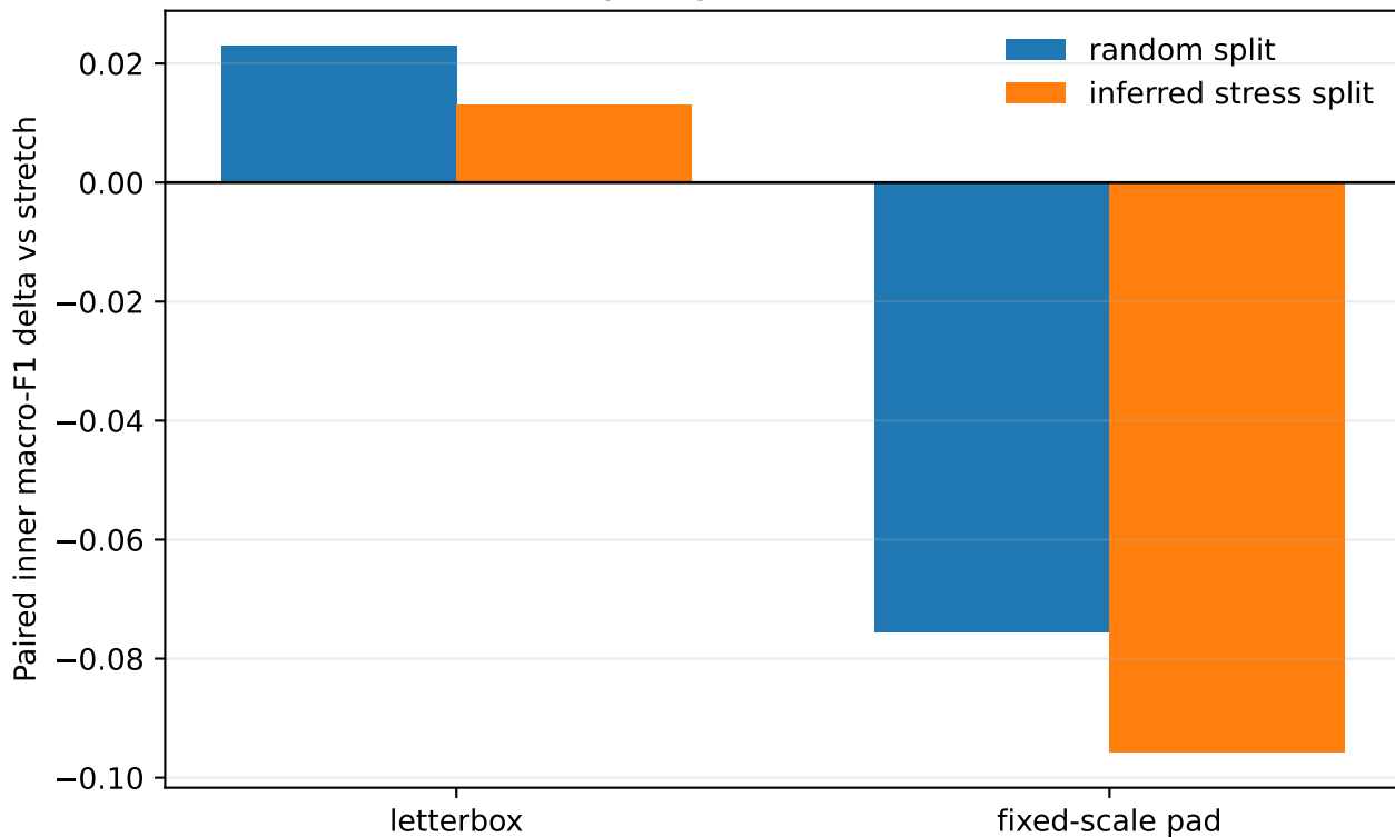
Geometry diagnostic (3 seeds, fold 0)
