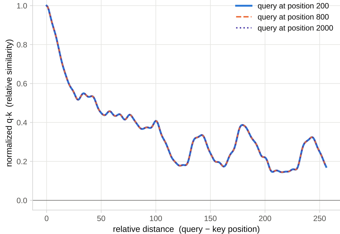
RoPE is relative — q·k depends only on the distance; curves at different absolute positions coincide
