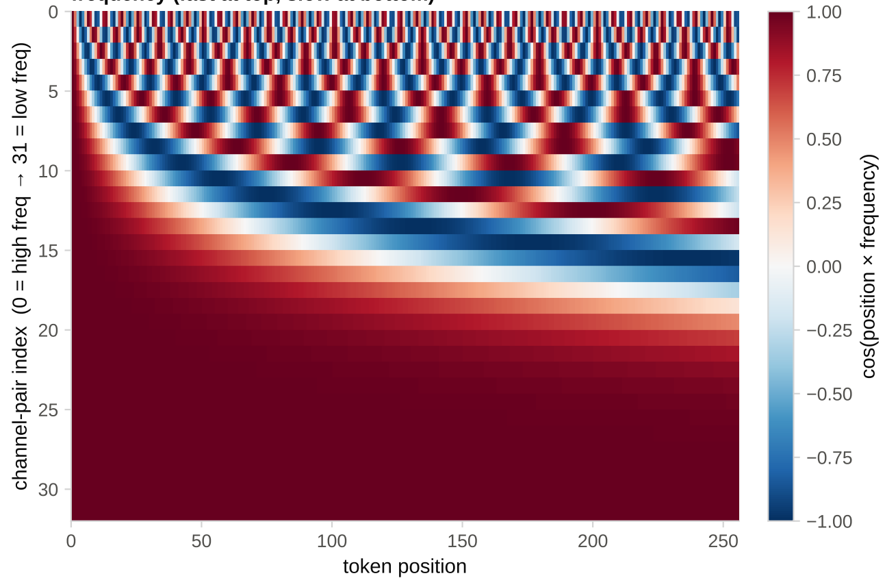
Multi-scale rotation — each channel pair spins at its own frequency (fast at top, slow at bottom)
