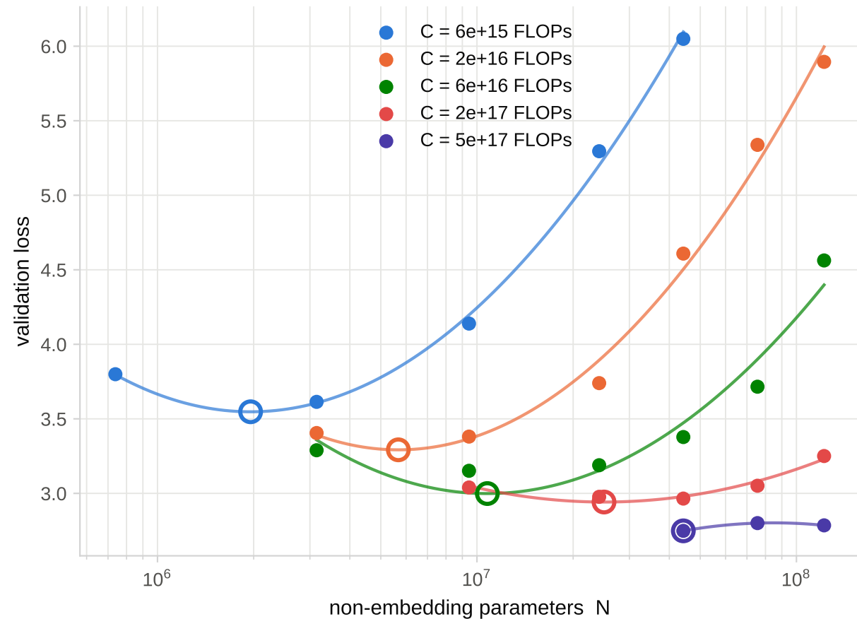
IsoFLOP profiles — the loss valley per compute budget (circle = compute-optimal size)
