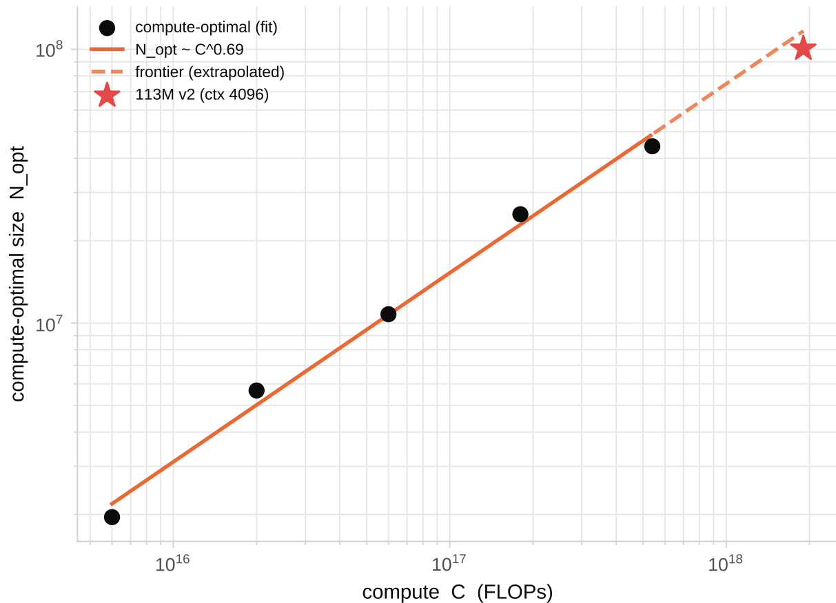
Compute-optimal frontier + the real 113M run (Chinchilla predicts an exponent \approx 0.5 )
