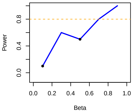
15777_G&gt;C, VC
