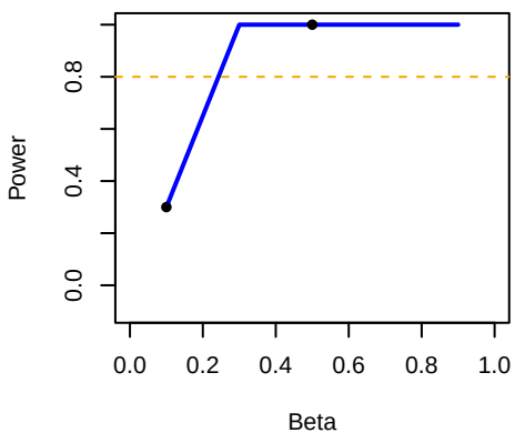
15777_G&gt;C, BE
