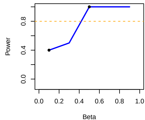
3071_T&gt;C, FB
