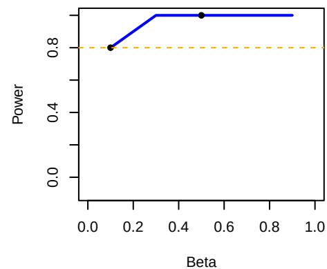
15777_G&gt;C, GC
