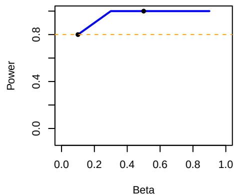
15777_G&gt;C, SQ
