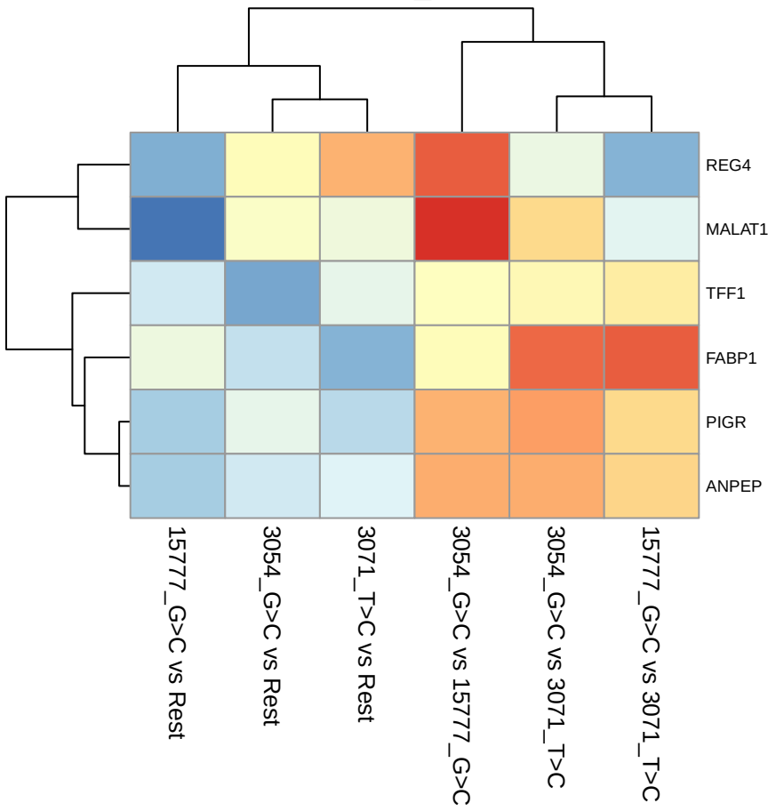
BE - test_statistic
