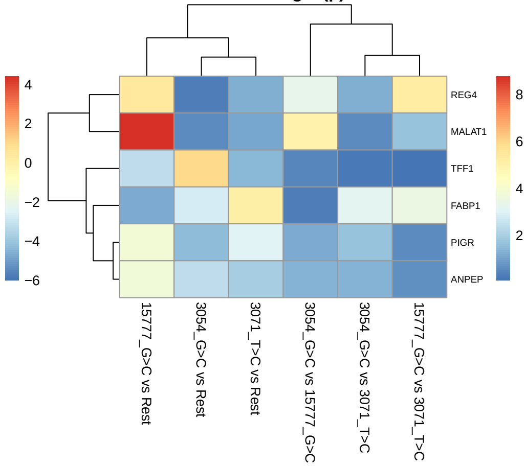
BE - -log10(p)
