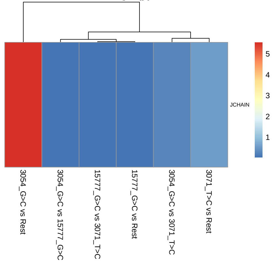
FB - -\log_{10}(p)
