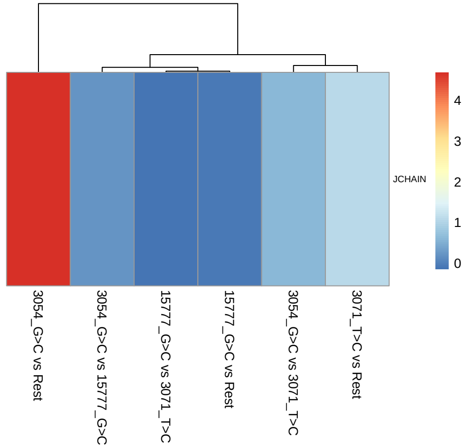
FB - test_statistic
