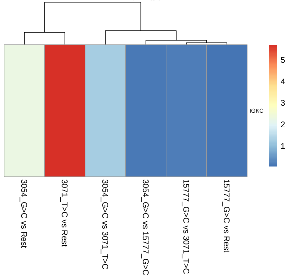
FB - -\log_{10}(p)
