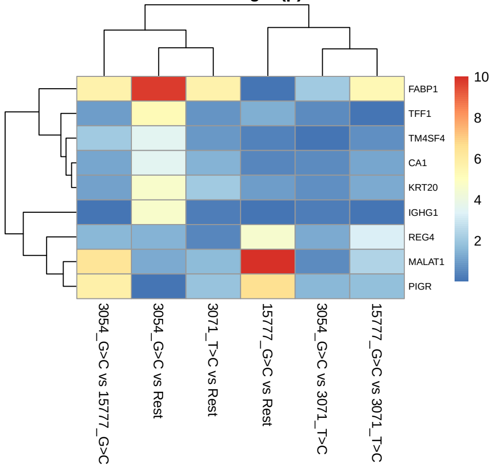
BE - -log10(p)
