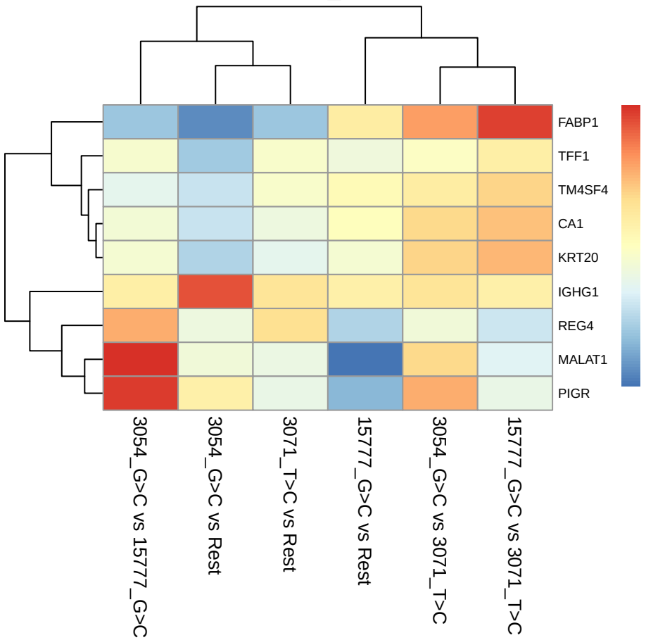
BE - test_statistic
