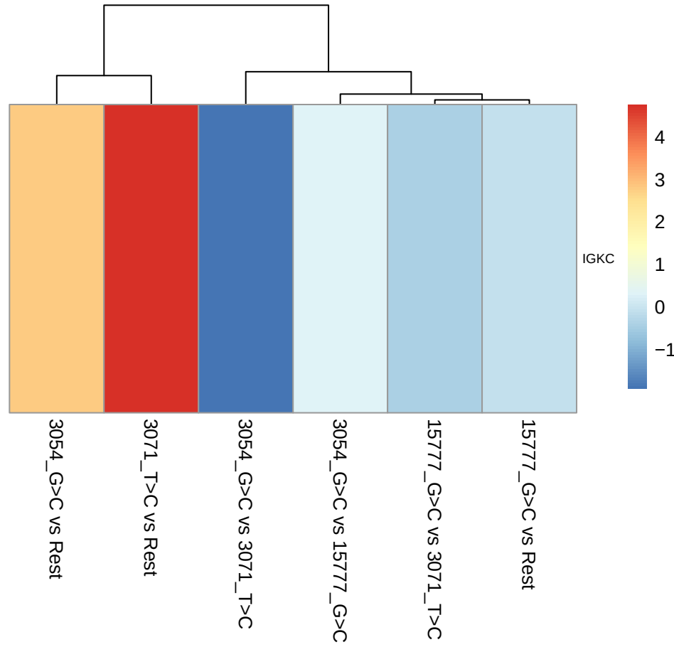
FB - test_statistic
