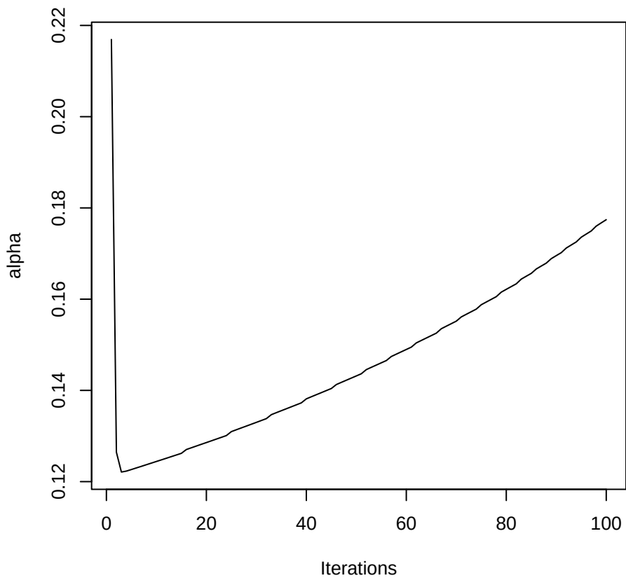
Change of alpha (Exclude start)
