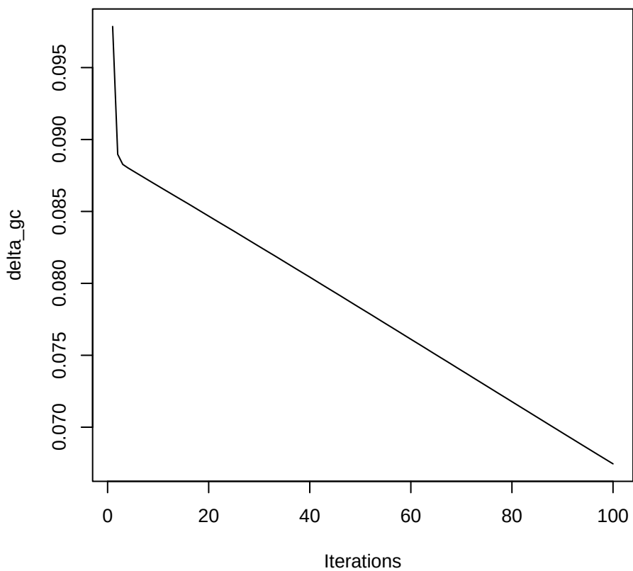
Change of delta_gc (Exclude start)
