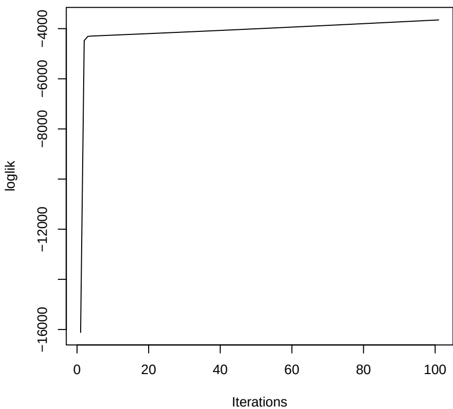
Change of Log Likelihood
