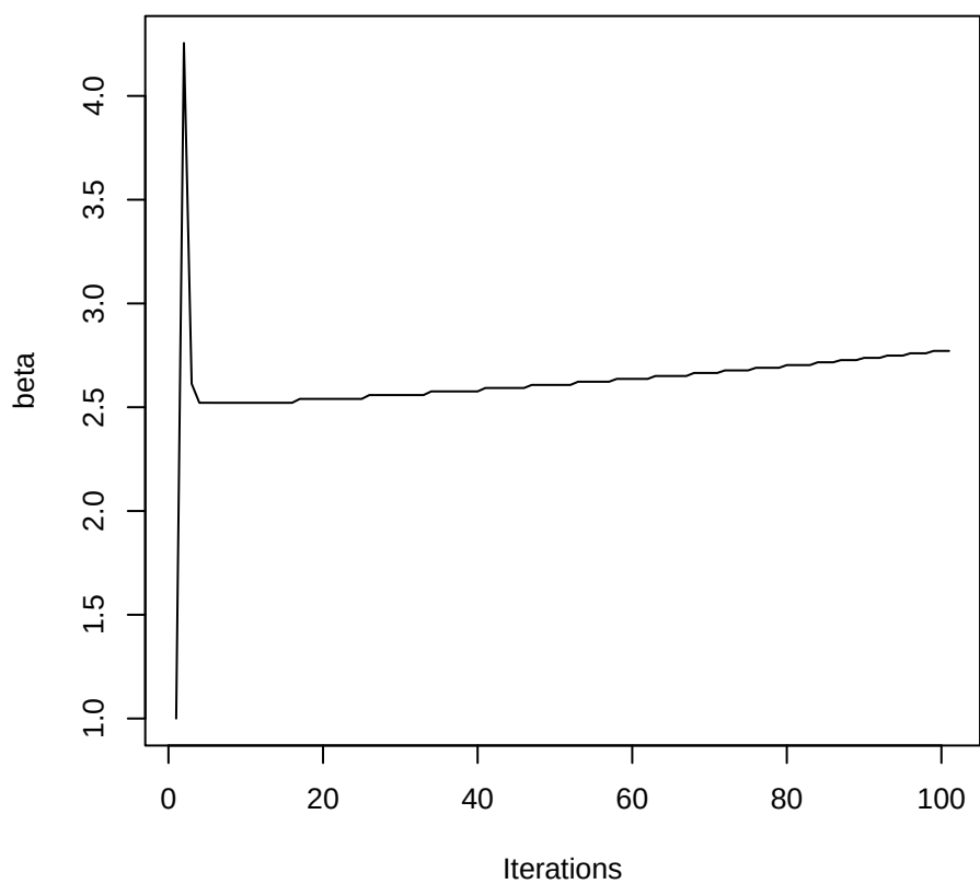
Change of beta
