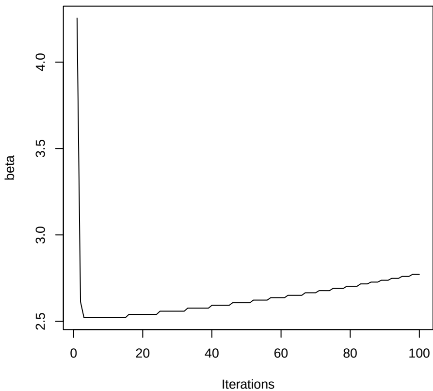
Change of beta (Exclude start)
