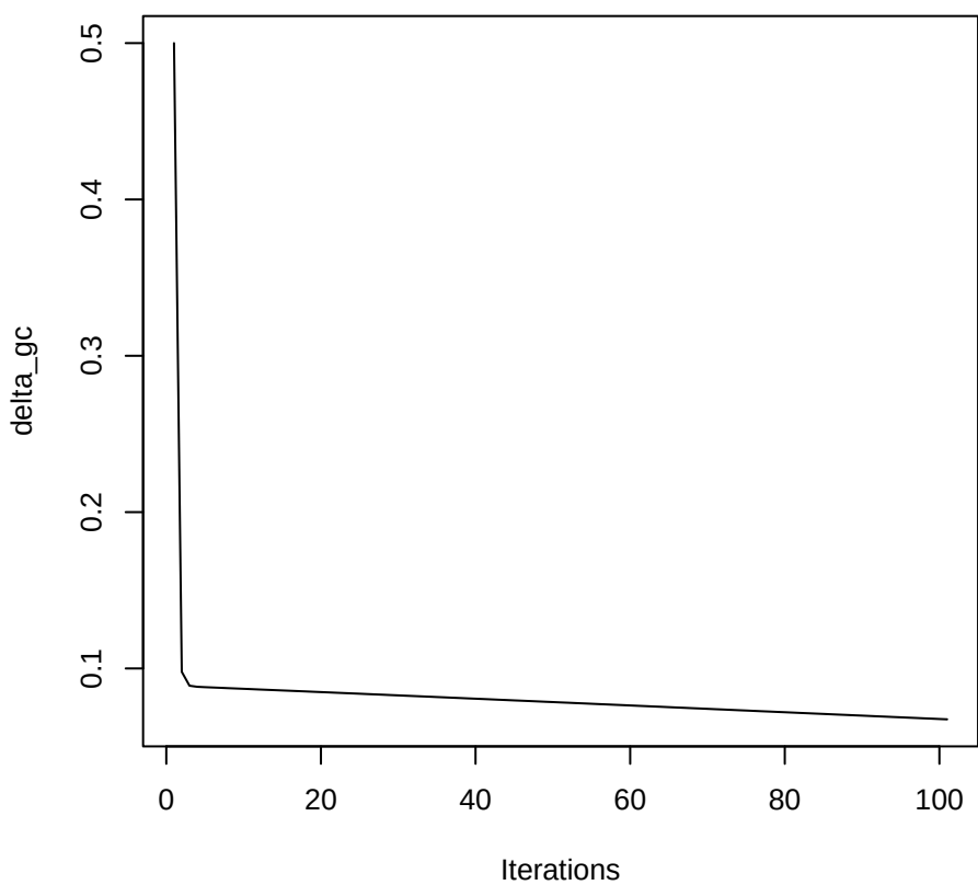
Change of delta_gc
