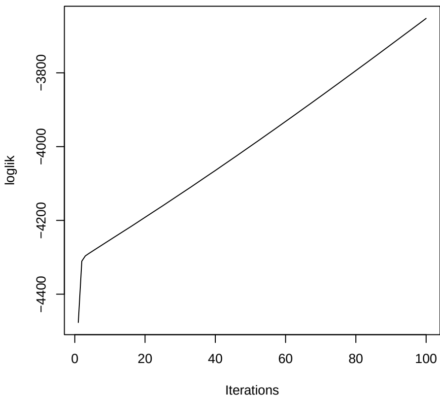
Change of Log Likelihood (Exclude start)
