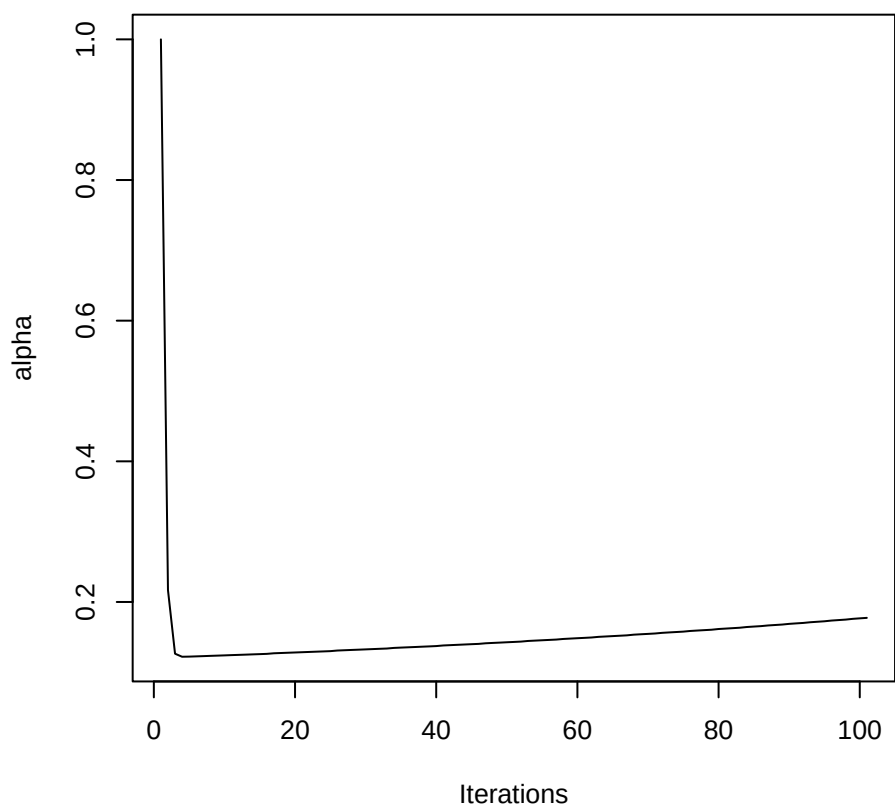
Change of alpha
