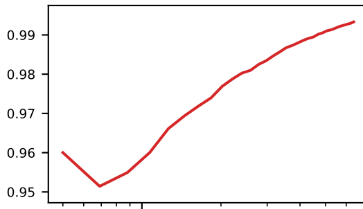
ns ( \theta_{\text{fid}}=0.983 )
