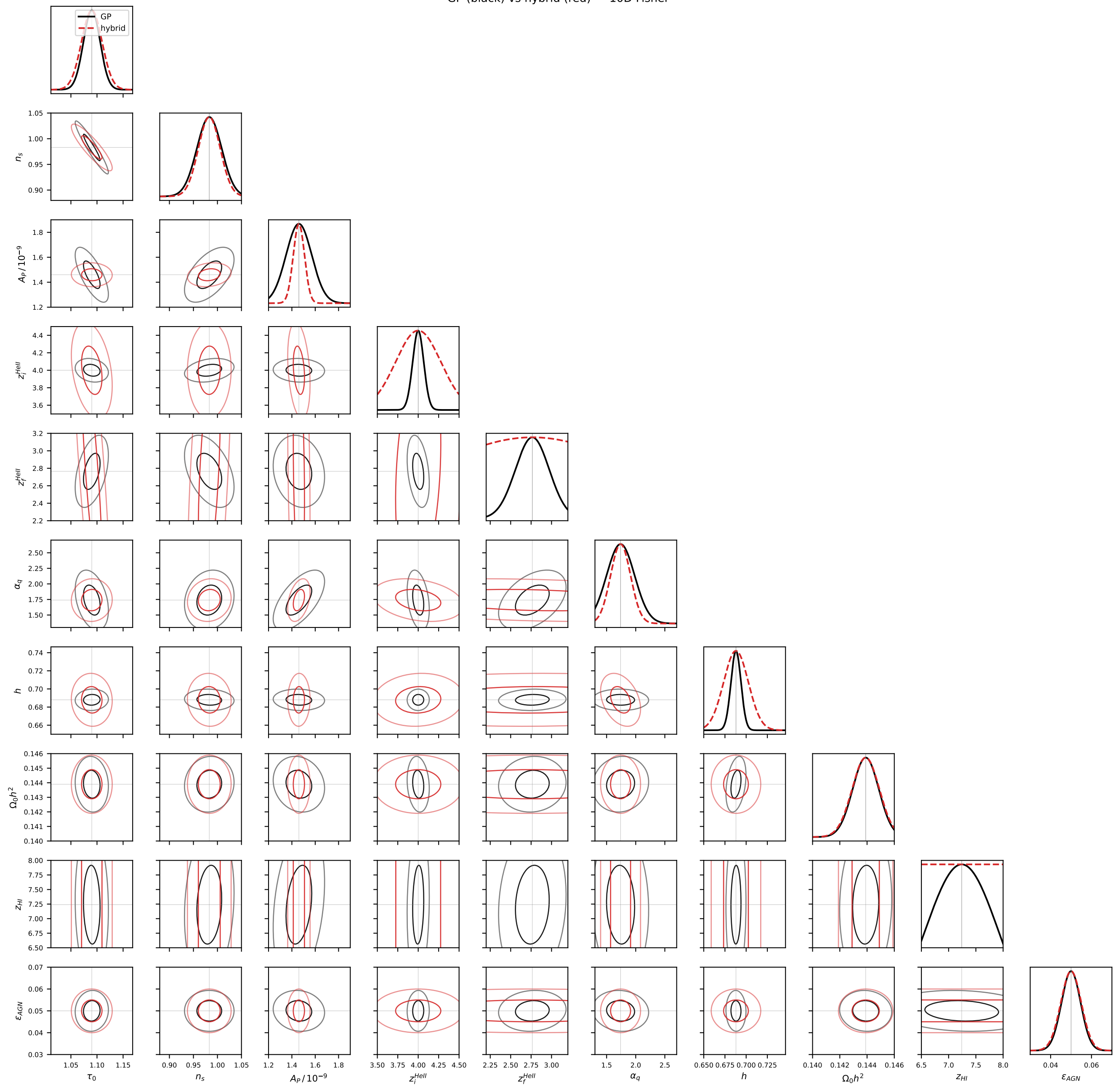
GP (black) vs hybrid (red) — 10D Fisher
