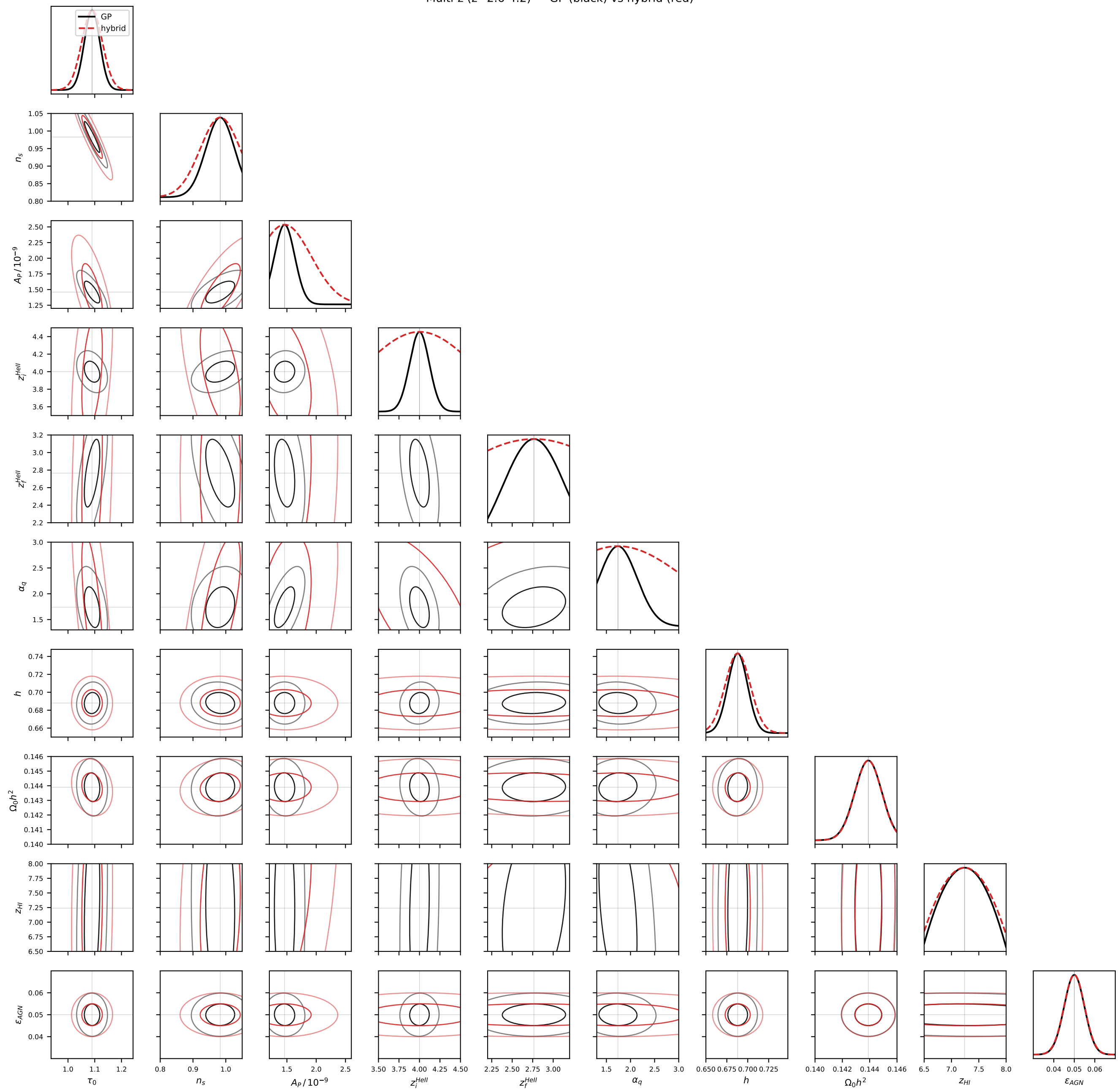
Multi-z (z=2.6-4.2) — GP (black) vs hybrid (red)
