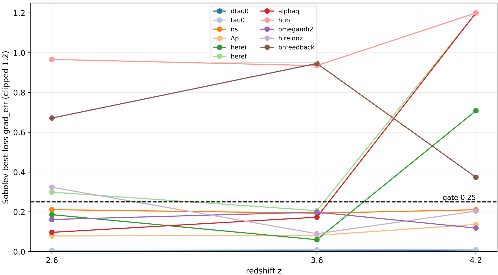
Redshift robustness of the derivative-faithfulness taxonomy (Sobolev fits)
