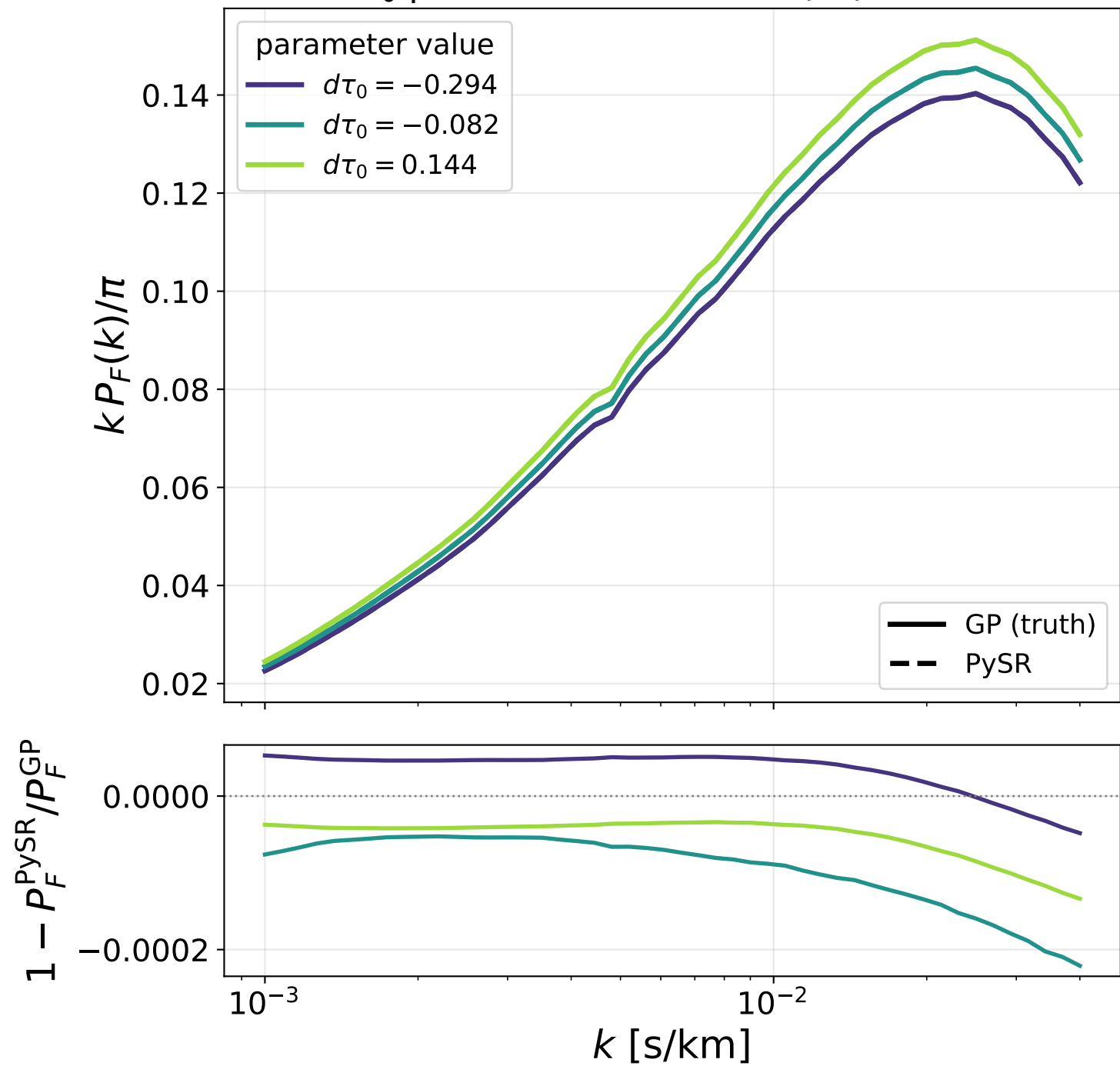
d\tau_0 predicted vs true P1D (LF), z = 3.6
