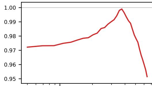
alphaq ( \theta_{\text{fid}}=1.74 )
