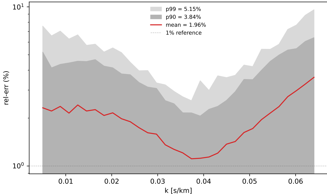
Multi-D Sobol hold-out (n=64, z=3.6, with pair coupling)
