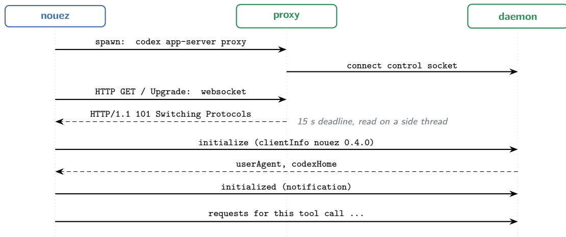
Figure 5: Opening a connection to the daemon. Bytes pass through the proxy unchanged.
