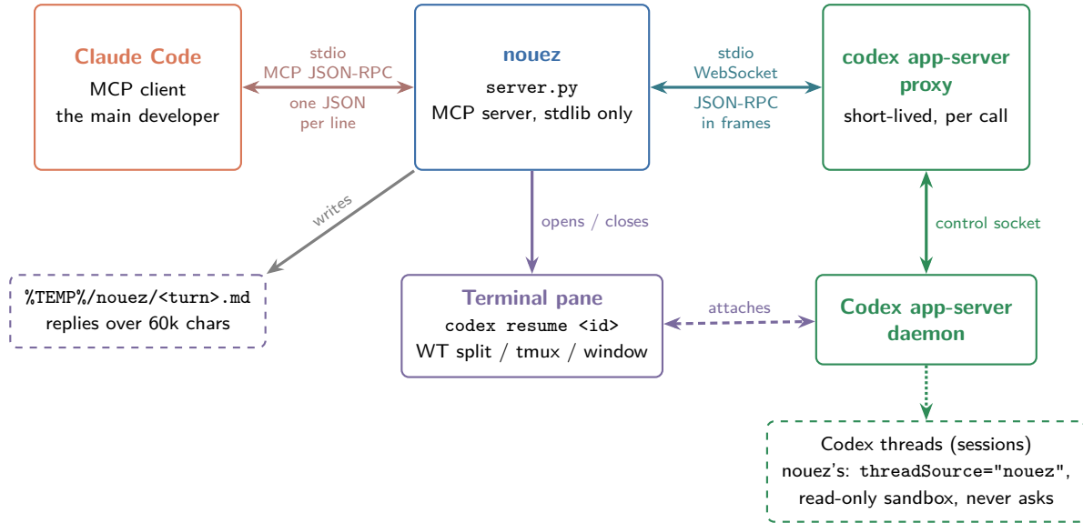
Figure 1: Components and links. Solid arrows carry messages; the terminal pane and nouez share a Codex session through the daemon, not through each other.
