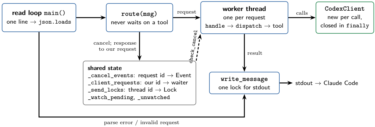
Figure 2: Threading model. Only write_message touches stdout, and logs go to stderr, so stdout carries nothing but MCP messages.
